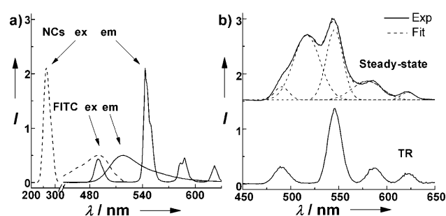
Figure 3. a) Excitation (dashed line) and emission (solid line) spectra of biotinylated NCs; excitation (dashed line) and emission (solid line) spectra of FITC. b) Steady-state and TR-PL (delay time = 100 \mu s , gate time = 1 ms) spectra of a mixture of 0.1 mM biotinylated NCs and 1 \mu M FITC under excitation at 290 nm. In steady-state detection, PL emissions of FITC and Tb^{3+} can be separated from the spectral deconvolution. The spectrum within 450–650 nm was best-fitted and deconvoluted to five Gaussian curves with peaks centered at 489, 520, 542, 585, and 623 nm.
